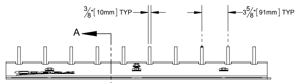
(B) FRONT VIEW SCALE NTS
