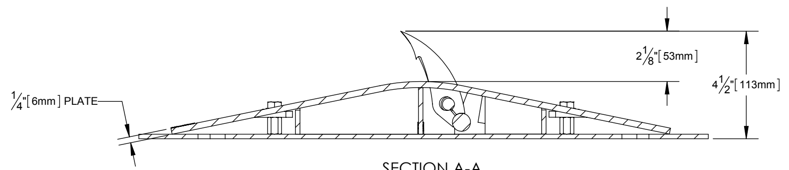
(C) SIDE VIEW SCALE NTS
